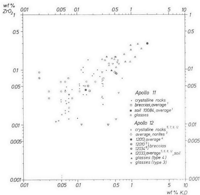
Fig. 8. ZrO_2 versus K_2O contents of glasses, igneous rocks, breccias, and soil from Apollo 11 and Apollo 12. Glass analyses of this work are represented by triangles. Data of Apollo 11 glasses and crystalline rocks are taken from LEVINSON (1970), Vols. 1 and 2. References for all other data are designated by superior numerals and are as follows: 1 COMPSTON et al. (1970); 2 WOOD (1970); 3 KEIL et al. (1971); 4 WAKITA and SCHMITT (1970); 5 LSPET (1970); 6 WAKITA et al. (1971); 7 ANNELL et al. (1971); 8 ROSE et al. (1971); 9 SMALES (1971); 10 MEYER et al. (1971); 11 HUBBARD et al. (1971); 12 BROWN et al. (1971); 13 BRUNFELT et al. (1971).
